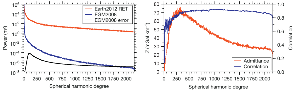
Figure 2 Power and cross power spectra of the Earth's radial gravity and topography. (Left) Power spectra of the topography (Earth2012 RET), geoid (EGM2008), and geoid error. (Right) Admittance and correlation spectra of the radial gravity and topography. The correlation spectrum is calculated using the spherical harmonic coefficients of the observed free-air gravity and gravity predicted from topography.
