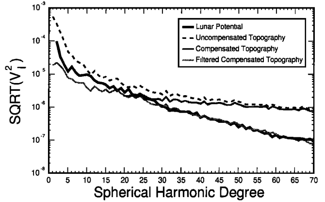
Figure 2. Square root of the power spectrum as a function of spherical harmonic degree, with \rho_c = 2900 \text{ kg/m}^3 and \rho_m = 3400 \text{ kg/m}^3 .
