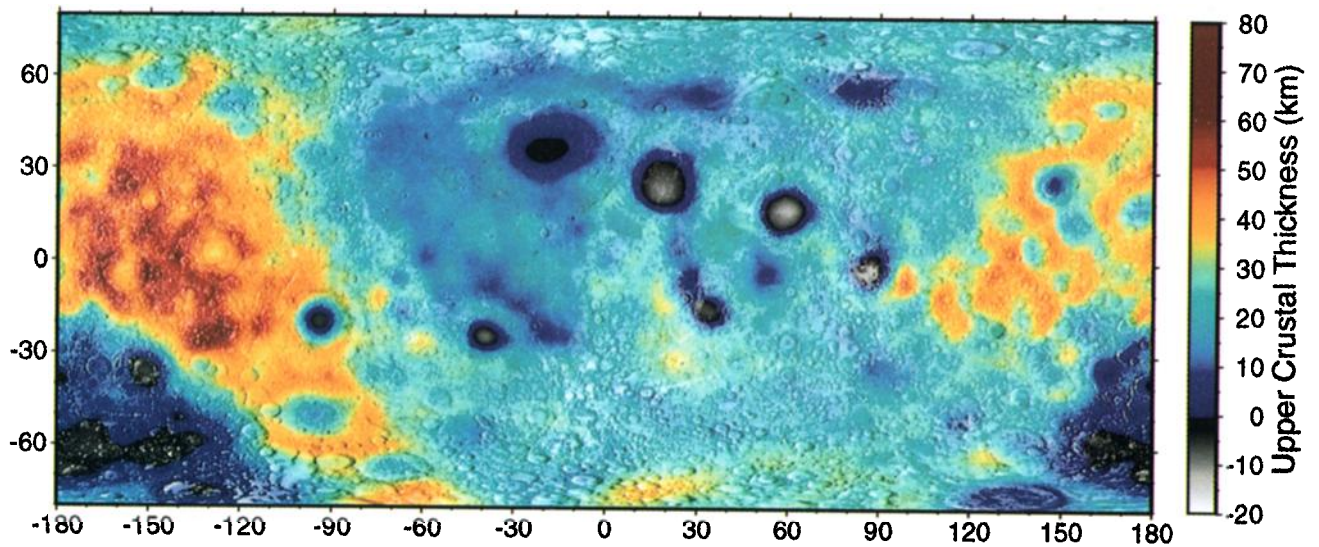
Plate 4. Upper crustal thickness minus mare fill for a dual-layered model with a constant thickness lower crust.
